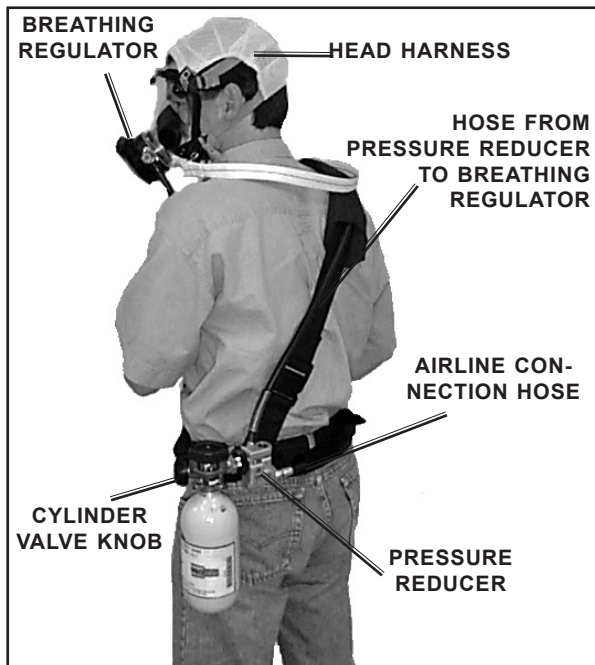
TYPICAL SKA-PAK PLUS CORROSION RESISTANT HARNESS REAR VIEW
