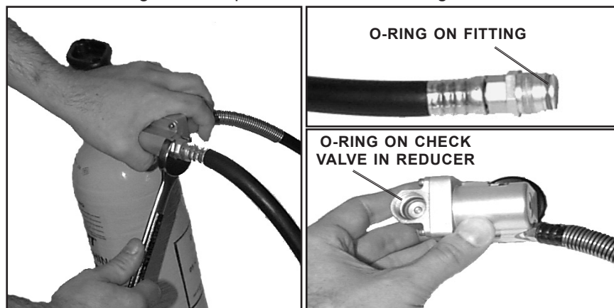
REPLACING THE AIRLINE CONNECTION HOSE
