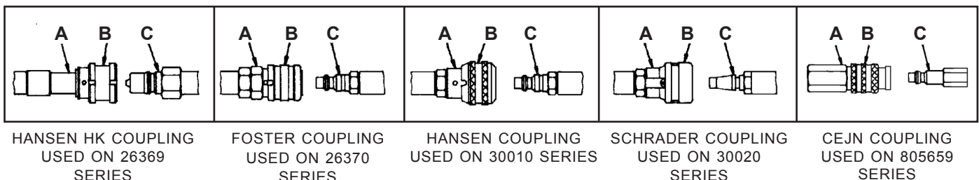
FIGURE 13 COUPLINGS USED ON SUPPLY HOSES
