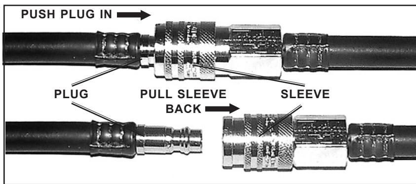
MODULAIR QUICK DISCONNECT FITTING FIGURE 7
